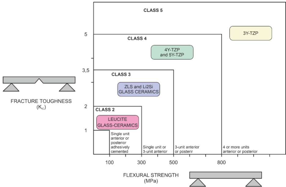
Figure 9. An overview ceramics classification according to ISO 6872:2015
